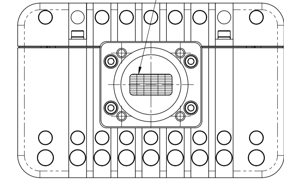
WR75 SEALED WAVEGUIDE OUTPUT
