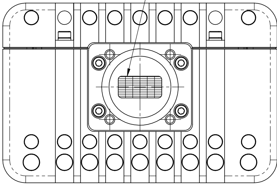
WR75 SEALED WAVEGUIDE OUTPUT
