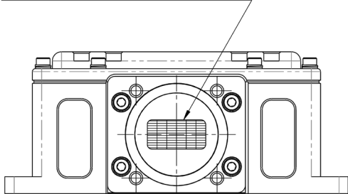
WR75 SEALED WAVEGUIDE OUTPUT
