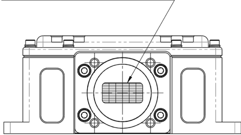
WR75 SEALED WAVEGUIDE OUTPUT
