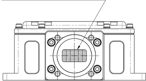
WR75 SEALED WAVEGUIDE OUTPUT
